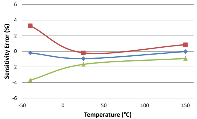
Sensitivity Error vs. Temperature
