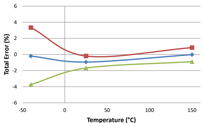
Total Error at I_{PR(max)} vs. Temperature
