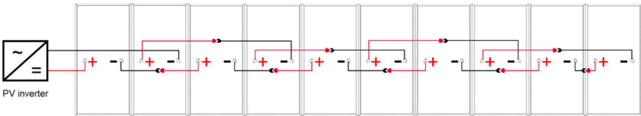
Portrait installation leapfrog wiring scheme even number of modules (eg. 10) with 1.67 m cable length
