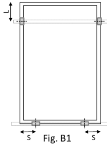
Fig. B1 Mounting rails perpendicular to the longer frame
