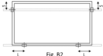
Fig. B2 Mounting rails parallel to the longer frame Clamp position on long & short frames
