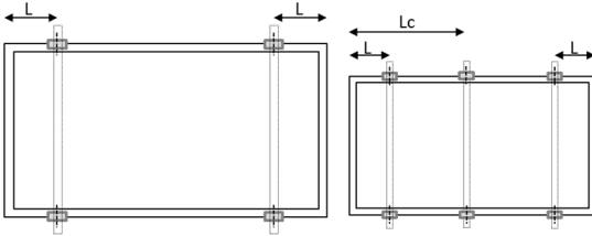
Fig. A1: Clamp position on long frames Mounting rails perpendicular to the longer frame
