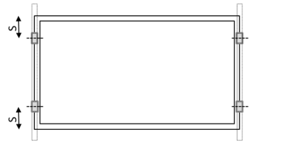
Fig. A2: Clamp position on short frames Mounting rails parallel to the shorter frame
