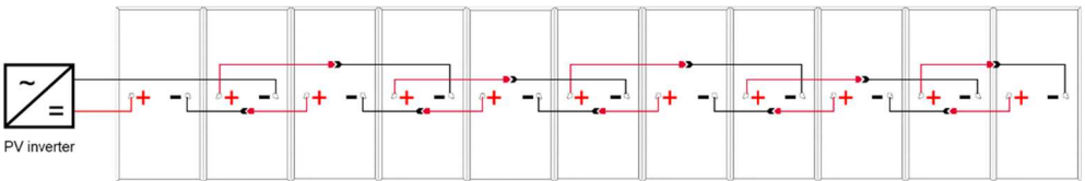
Portrait installation leapfrog wiring scheme odd number of modules (eg. 11) with 1.67 m cable length
