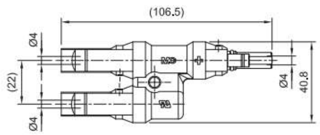
MC4 male branch connector
