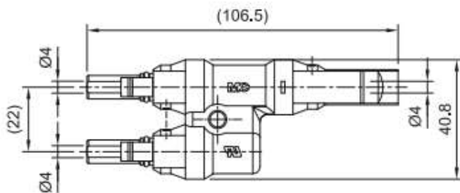
MC4 female branch connector
