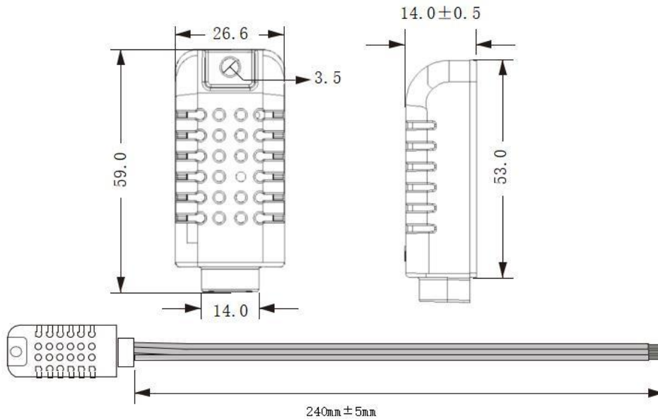
Figure 12. AM2301B sensor encapsulation (unit: mm not specified tolerance: ± 0.2 mm)
